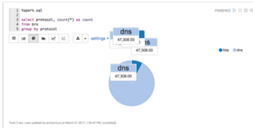
Figure 4.2. Bro Protocols
