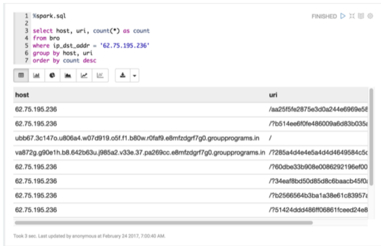
Figure 4.9. x-dosexc Requests
