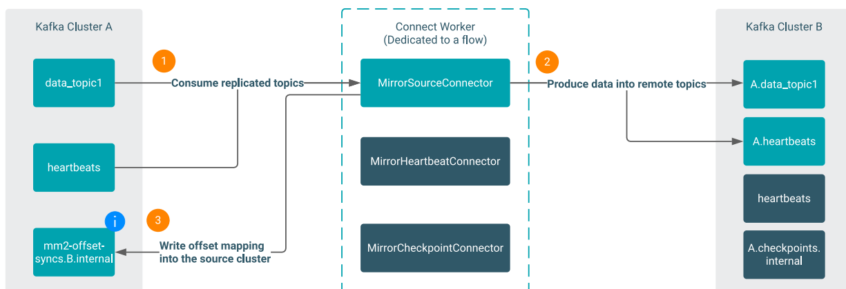
Figure 6: MirrorSourceConnector
