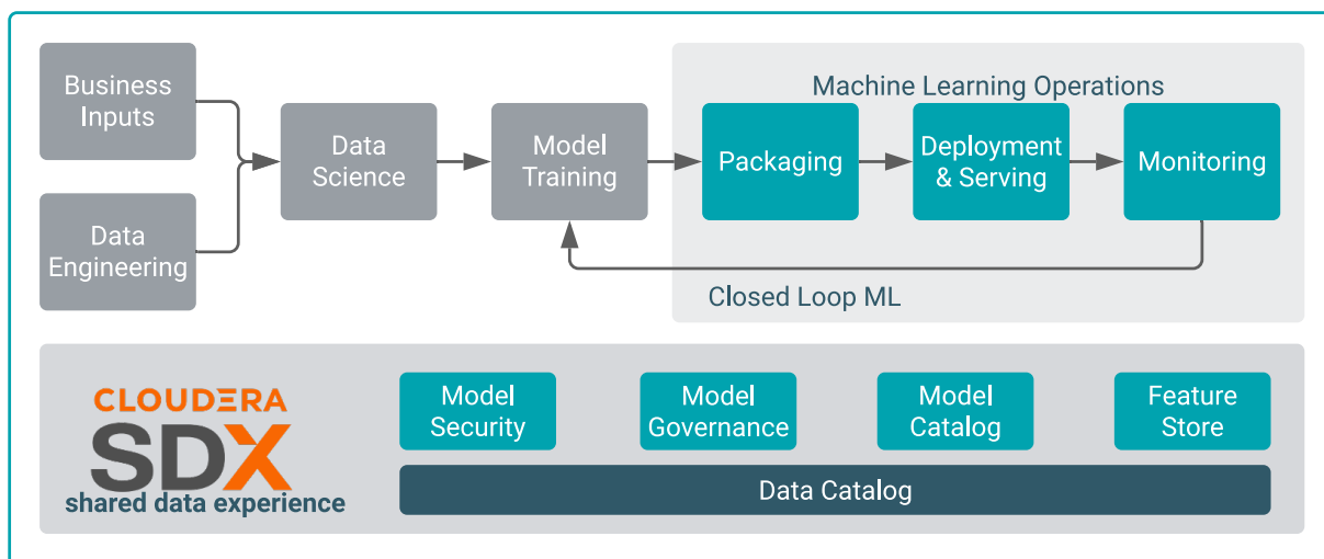
Figure 1: Production ML Workflow
