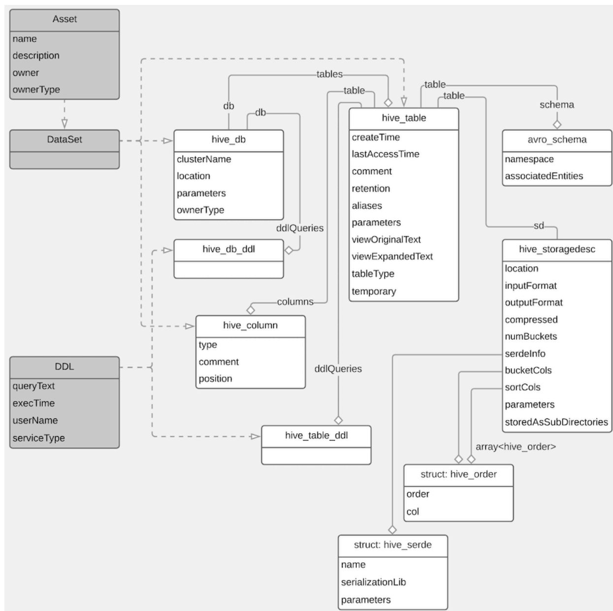
Figure 2: Atlas Entity Types for Hive Server 2 Processes
