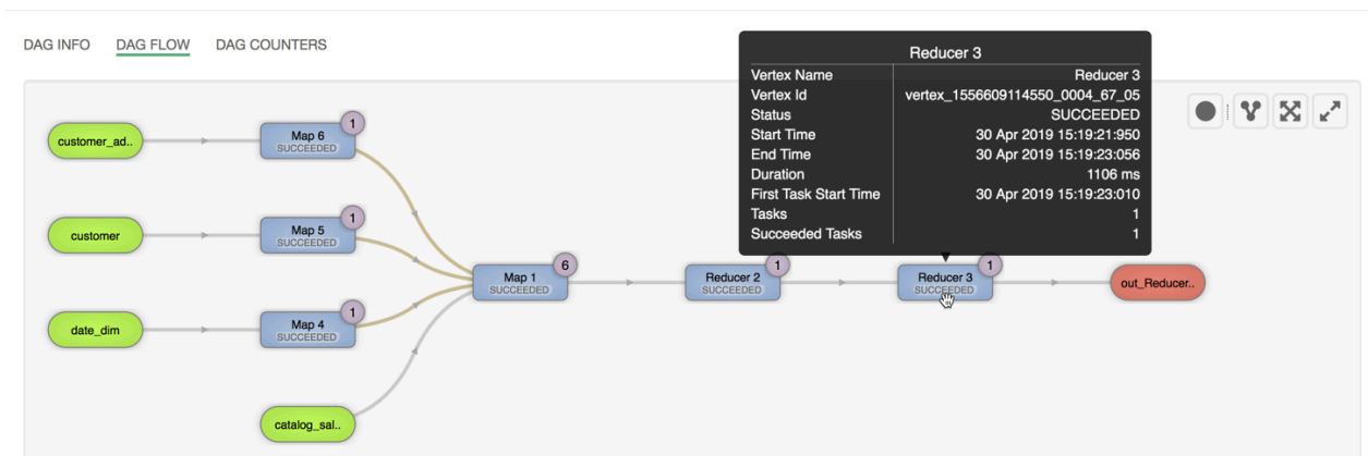
Figure 5: DAG flowchart
