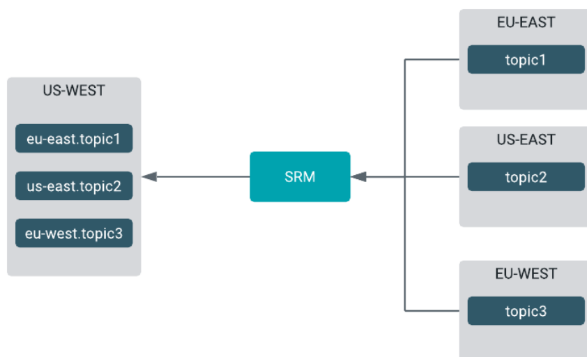
Figure 13: Fan-in Replication Flow
