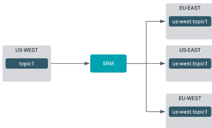
Figure 14: Fan-out Replication Flow
