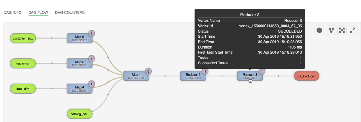
Figure 5: DAG flowchart
